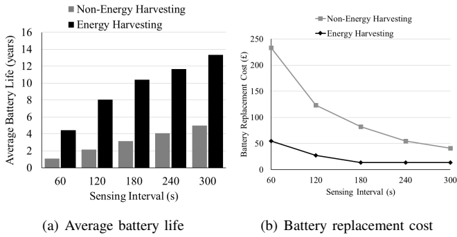
Fig. 1. Average battery life and battery replacement cost comparison between EH and non-EH environment against sensing interval
