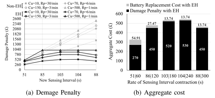
Fig. 2. Damage penalty against new sensing interval and aggregate cost in energy harvesting environment against the rate of sensing interval contraction
