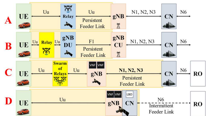
Figure 2 – Possible T/NT architectures of interest in the ITA NTN project.
